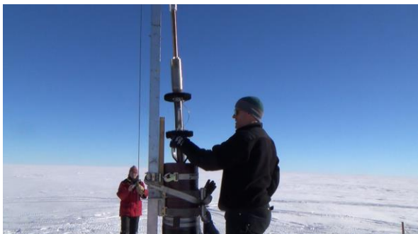
Ryan Bay and Elizabeth Morton deploy borehole logging instruments at Siple Dome. Photo credit: Joseph Talghader.
