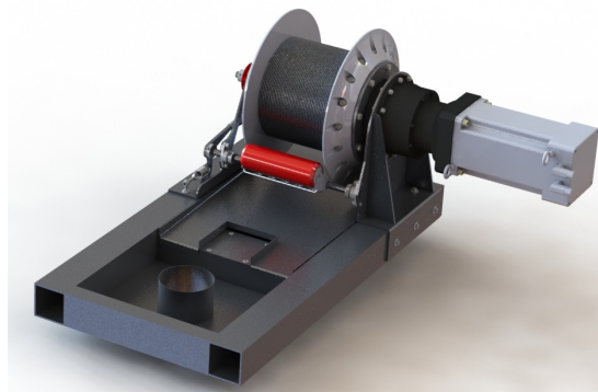
(left) Proposed layout of the 700 Drill inside of a modified MAST Tent. (right) 700 Drill winch drum, motor and base design. Credit: Grant Boeckmann
