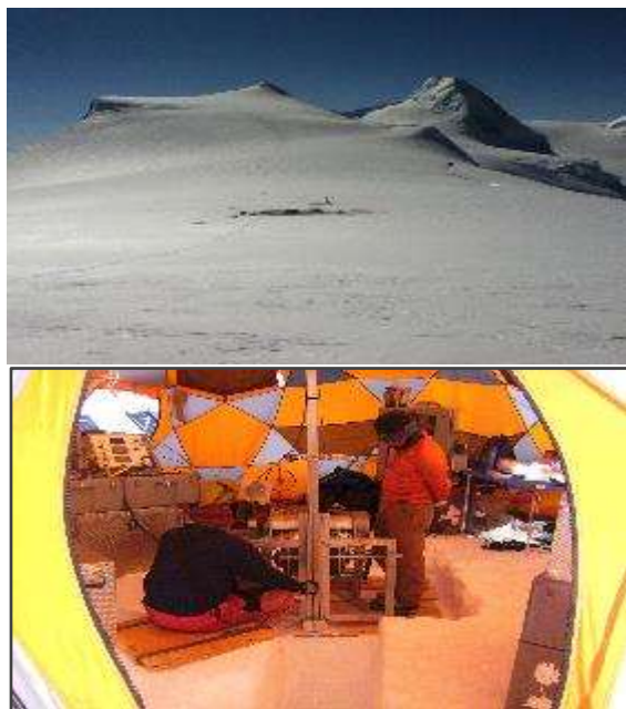
Scientific drilling on the Mt. Hunter Plateau of Denali provides a 2,000-year record of precipitation and atmospheric circulation in Central Alaska. Drilling at this site was accomplished by wind and solar energy without the need for gas-fueled generators. Photo credit: Top) Seth Campbell, CRREL; Bottom) Dom Winski, Dartmouth
