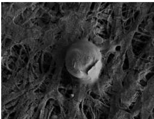
Caption: Microbial ecosystems have been found under the West Antarctic Ice sheet (Christner et al, 2014). This photo shows a coccoid-shaped microbe with an attached sediment particle from subglacial Lake Whillans. Photo credit: Trista Vick-Majors .
