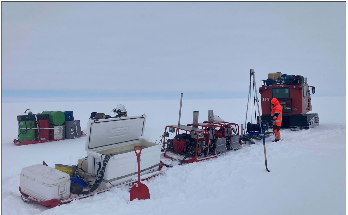
(Right) RAM Drill operations at WAIS Divide, Antarctica. Credit: Tanner Kuhl. (Bottom) Small Hot Water Drill (SHWD) traverse setup. The SHWD was used at Lower Thwaites Glacier to drill thirty-two holes for seismic shot hole work. Credit: Tanner Kuhl.
