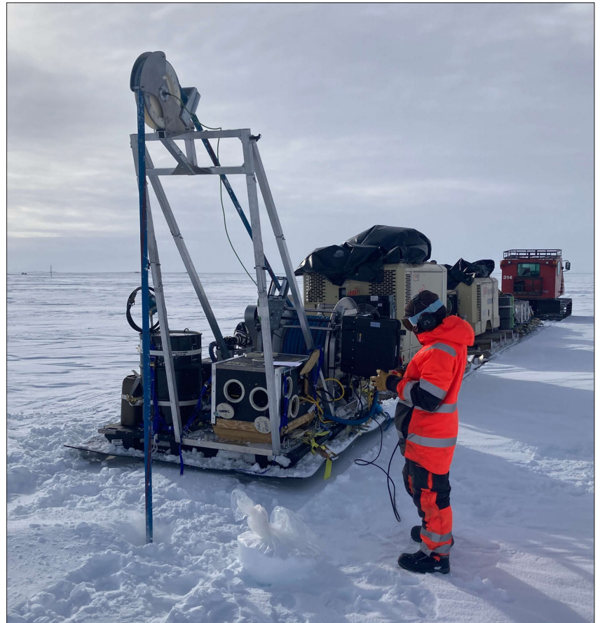
(Right) RAM Drill operations at WAIS Divide, Antarctica. Credit: Tanner Kuhl. (Bottom) Small Hot Water Drill (SHWD) traverse setup. The SHWD was used at Lower Thwaites Glacier to drill thirty-two holes for seismic shot hole work. Credit: Tanner Kuhl.
