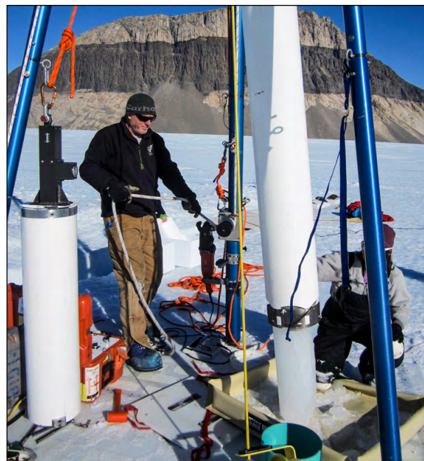
Driller Mike Jayred operating the Blue Ice Drill on Taylor Glacier.
