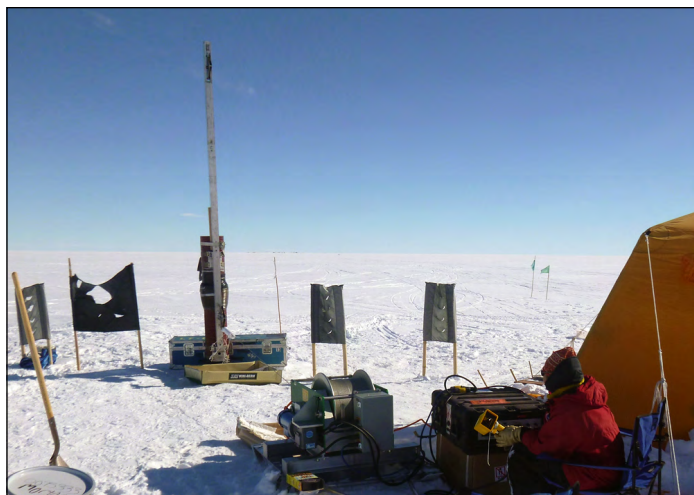
The intermediate depth logging winch in operation at Siple Dome. For more info about the winch, visit: http://www.icedrill.org/equipment/
