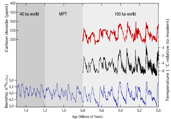
The 100,000-year 'sawtooth' variability in Antarctic climate over the last 800,000 years is mirrored by generally, similar variability in atmospheric carbon dioxide (as well as methane and nitrous oxide, not shown) and global ice volume inferred from deep ocean oxygen isotope records from marine calcium carbonate. Whether Antarctic climate followed the ice volume record prior to this time, when ice volume records are dominated by a 40,000-year period, is not known, neither are the mean levels of greenhouse gases and the temporal variability of those levels. Figure from Severinghaus et al. (2013).
