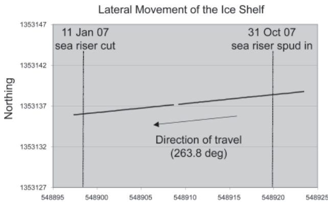
Fig. 1 – Distance and direction of total lateral movement of the MIS Project Drill Site located on the McMurdo Ice Shelf.
