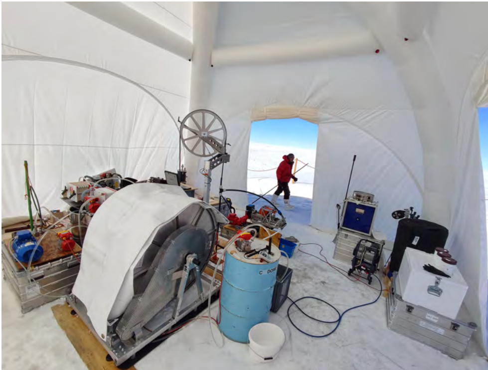
Figure 1. The RADIX system is housed in an inflatable, windproof shelter (dimensions: 7 m × 7 m × 5 m) from AXION ( https://www.axion4event.com , last access: 27 February 2023).
