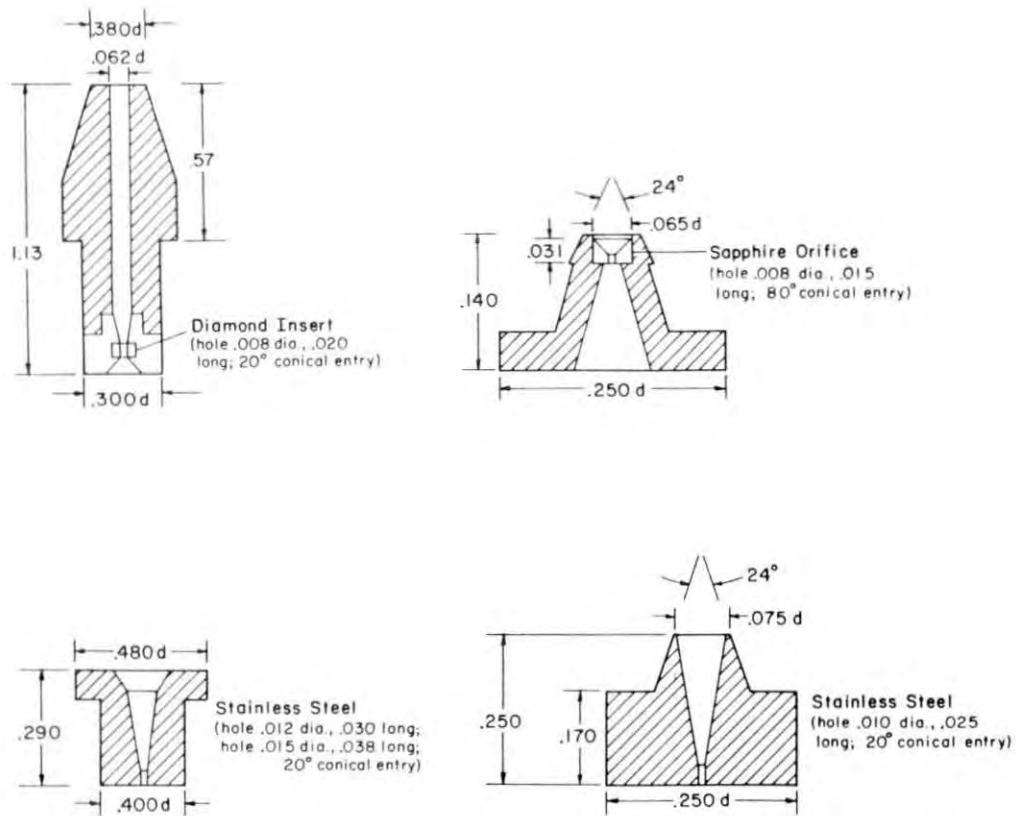
Figure 4. Examples of nozzles for high pressure water jet cutting.
