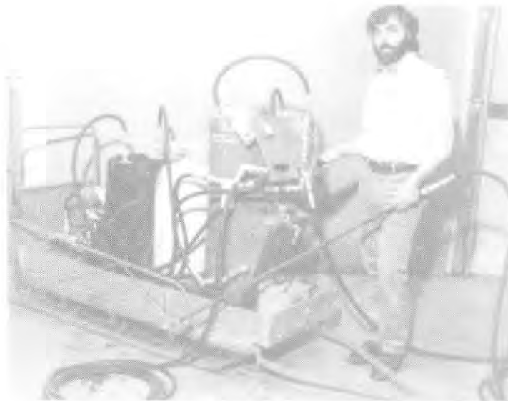
Figure 10. Hot-water drill packaged on a small toboggan for work at remote sites on arctic sea ice.
