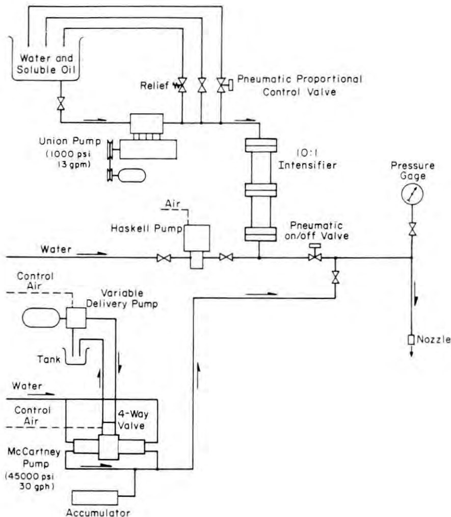
Figure 3. Example of equipment for high pressure water jet cutting.
