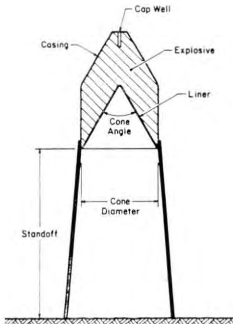
Figure 1. Basic features of a typical rotationally symmetrical shaped charge.
