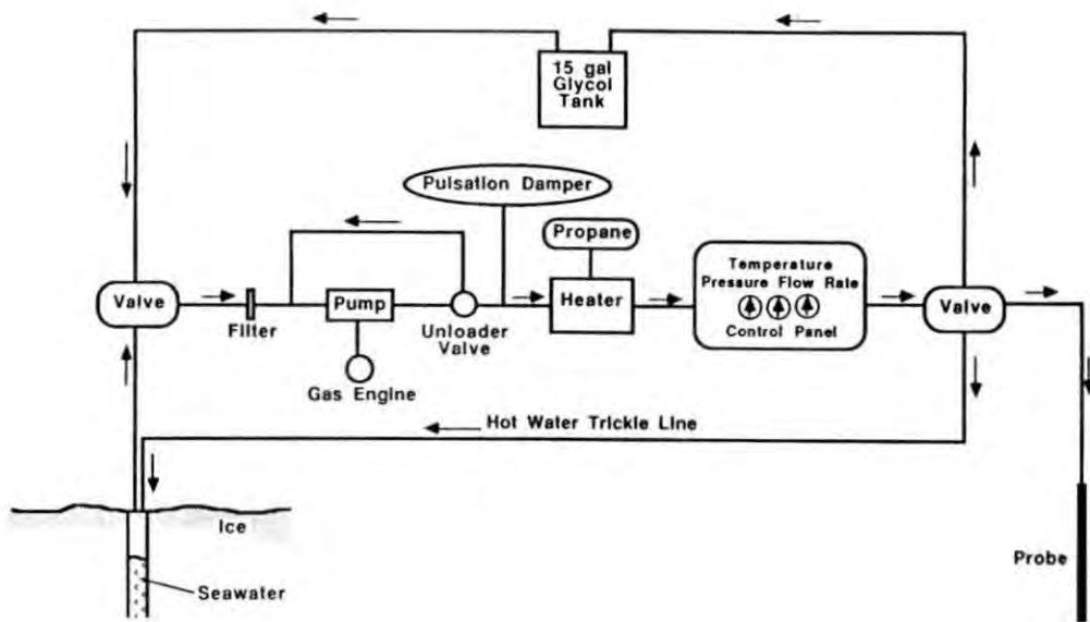
Figure 8. Example of equipment for hot-water drilling (Tucker et al., in press).
