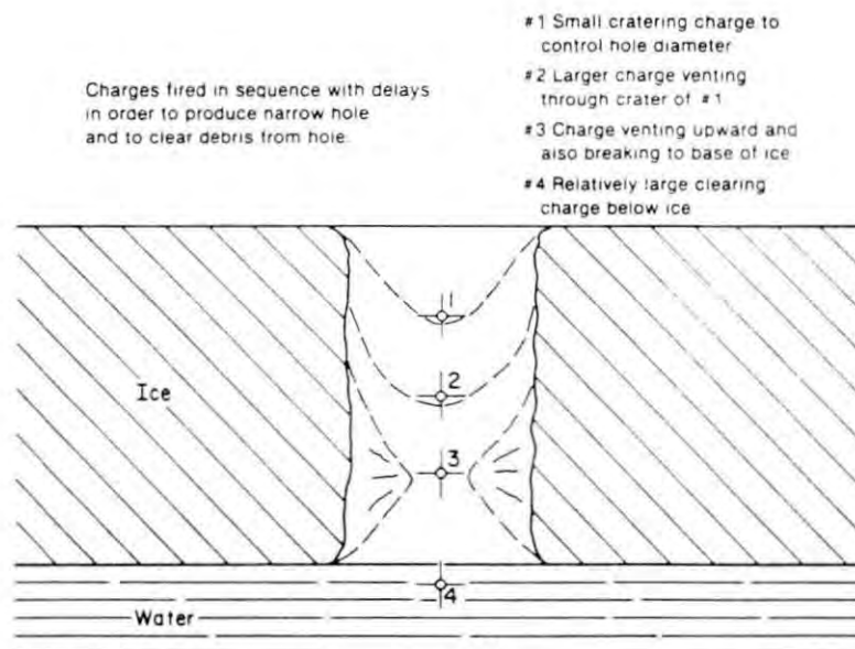
Figure 7. Use of delay deck charges to break a narrow shaft through very thick ice.
