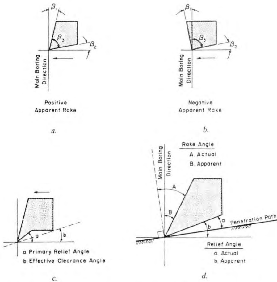
Figure 20. Tool angles for chisel-edge drag bits on rotary boring heads. The tool angles are normally specified in accordance with (a) (Mellor 1976).
