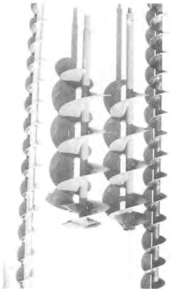
Figure A14. Auger flights with pitch and stem diameter suitable for ice drilling
