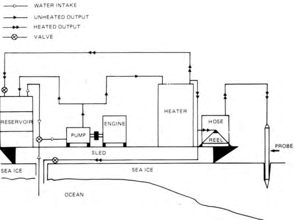
Figure 9. Example of equipment for hot-water drilling (Poplin et al., in press).
