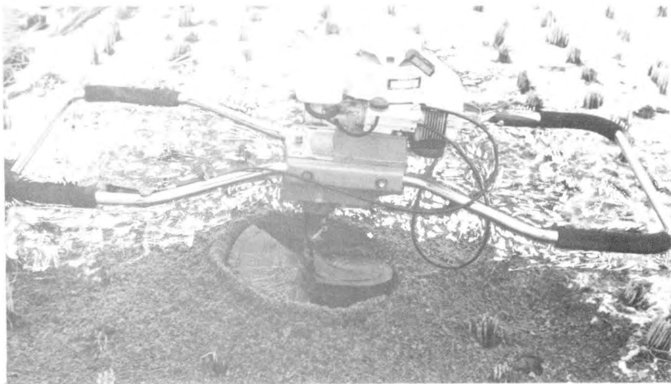
Figure A11. Gasoline drive unit (3.5-hp post-hole digger) used to turn a 14-in.-diam auger in frozen ground. The butterfly handles are considered a hazard.
