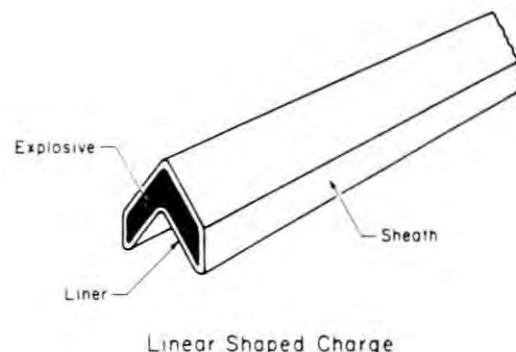
Figure 2. Linear shaped charge.
