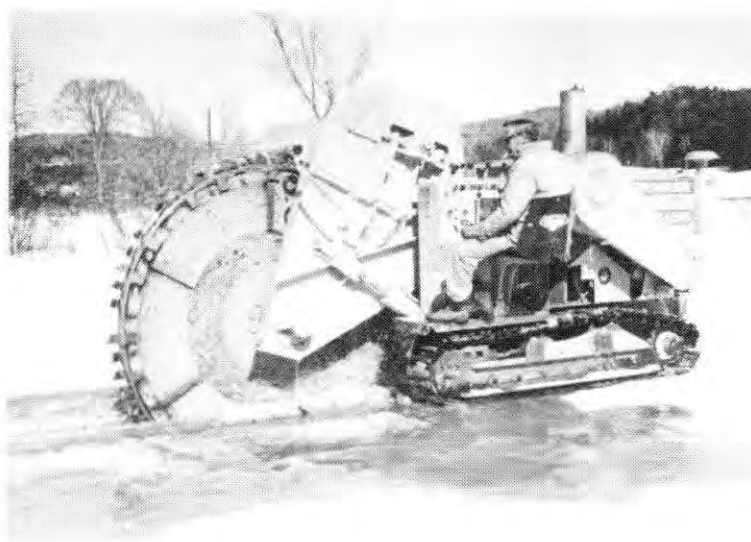
Figure 16. Vermeer disc saw cutting lake ice.
