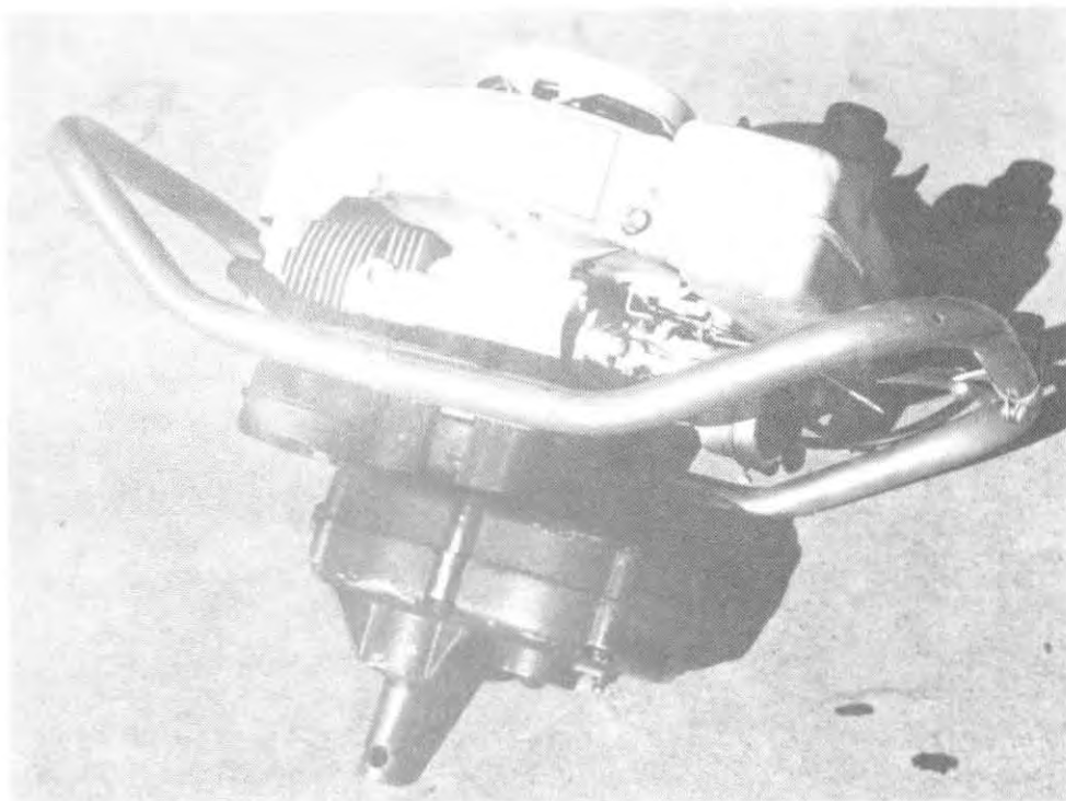
Figure A10. Gasoline drive unit, showing gear case.
