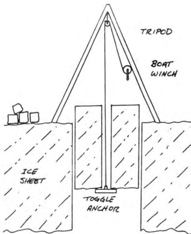
Figure 19. Simple tripod for lifting ice blocks (Hansen 1986).
