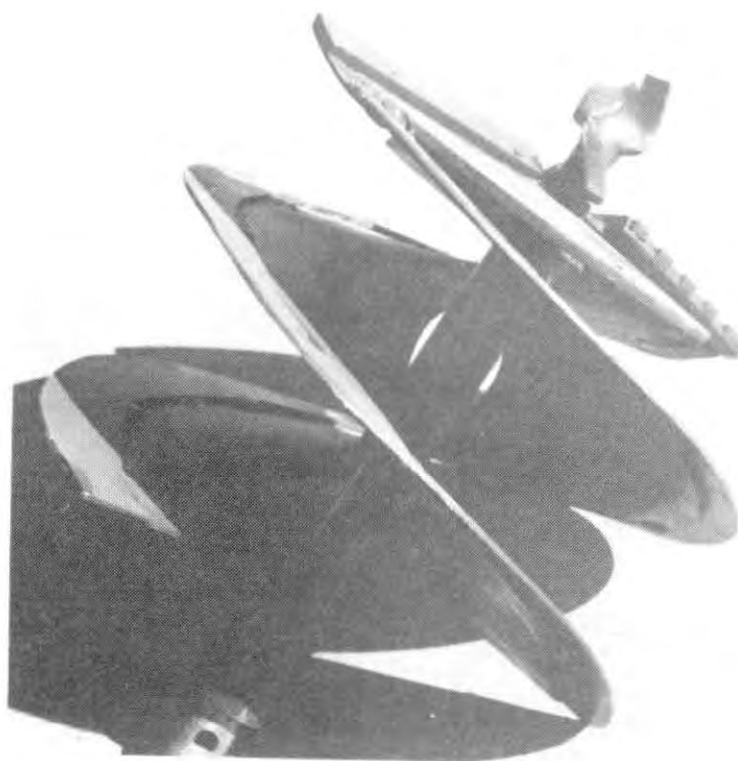
Figure 26. Fourteen-inch-diameter auger for drilling in frozen soil. The two-wing bit with pilot could easily be modified for ice drilling by using sharp steel cutters instead of the carbides shown here.
