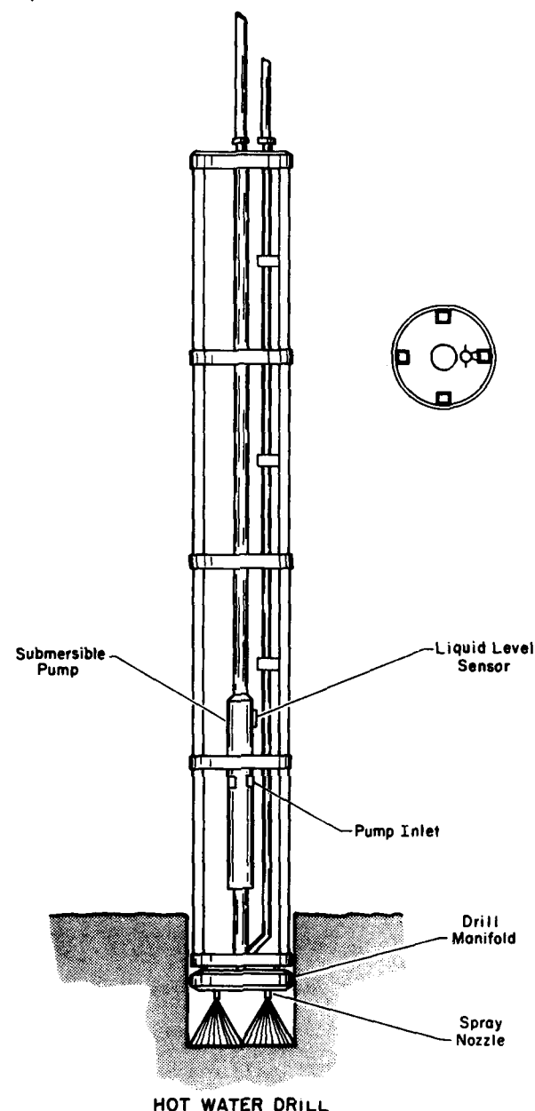
Figure 4. Hot-water drill.
