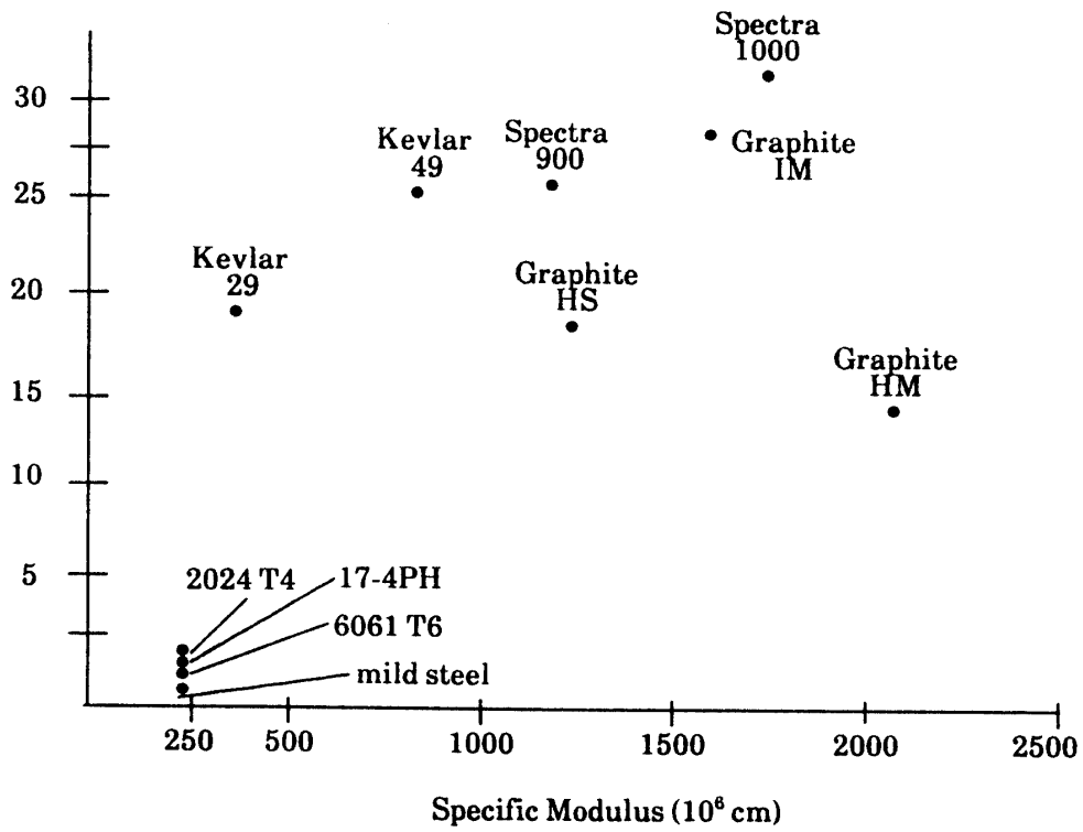
Fig. 2. Tensile strength of various drill cable materials.
