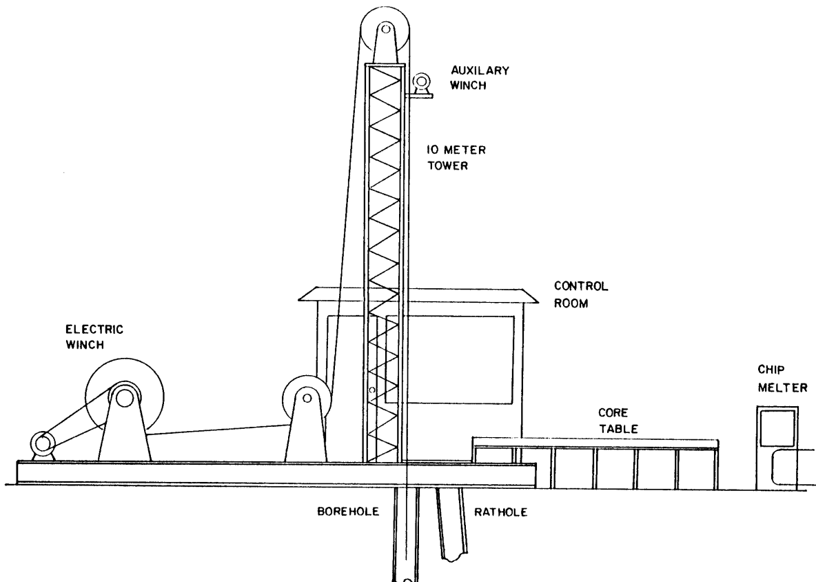
Fig. 3. Possible future design of surface handling equipment for the PICO 13.2 cm ice coring drill.
