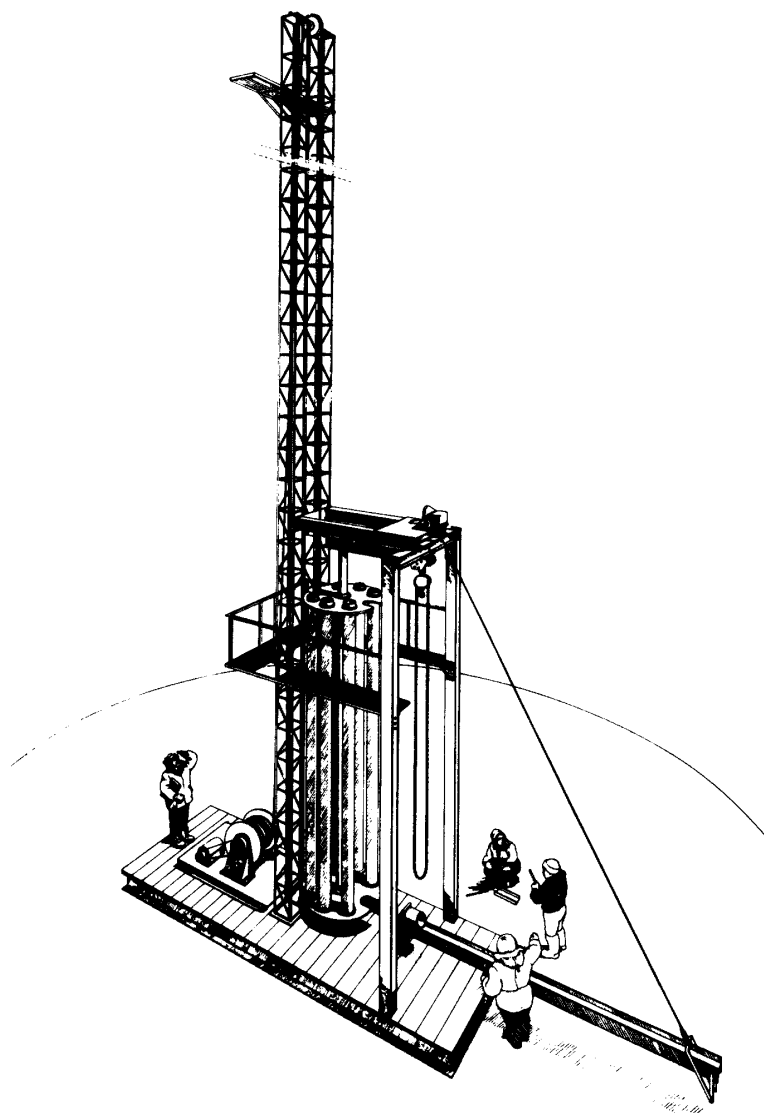
Fig. 4. Tower and surface equipment for the PICO 13.2 cm ice coring drill.
