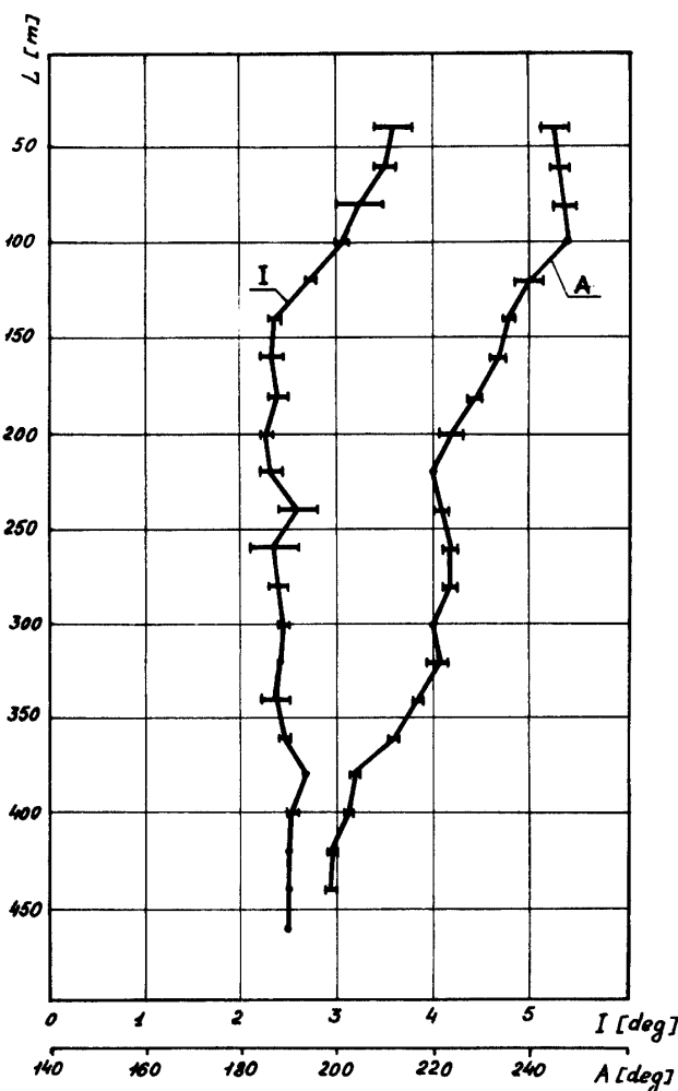
Fig. 6. Inclination of bore-hole 461.6 m versus depth L: I-inclination, A-magnetic azimuth.
