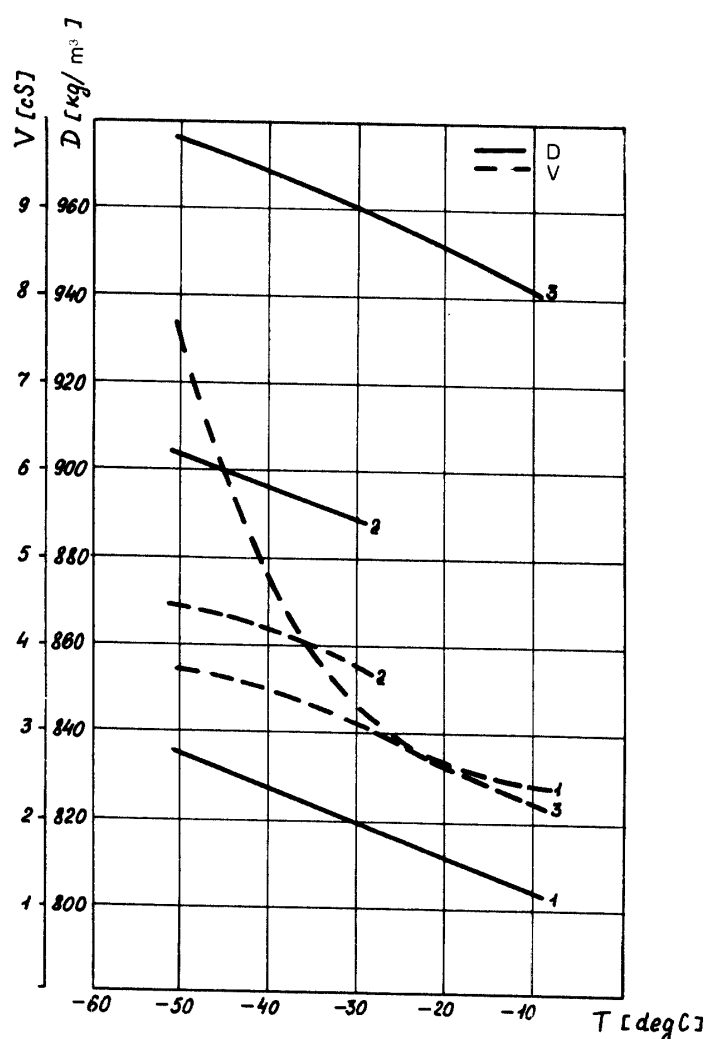
Fig. 5. Hole liquid density D and viscosity V versus temperature T : 1-kerosene TS-1, 2-mixture of kerosene TS-1 and 5% vol. freon-11, 3-mixture of kerosene TS-1 and 20% vol. freon-11.
