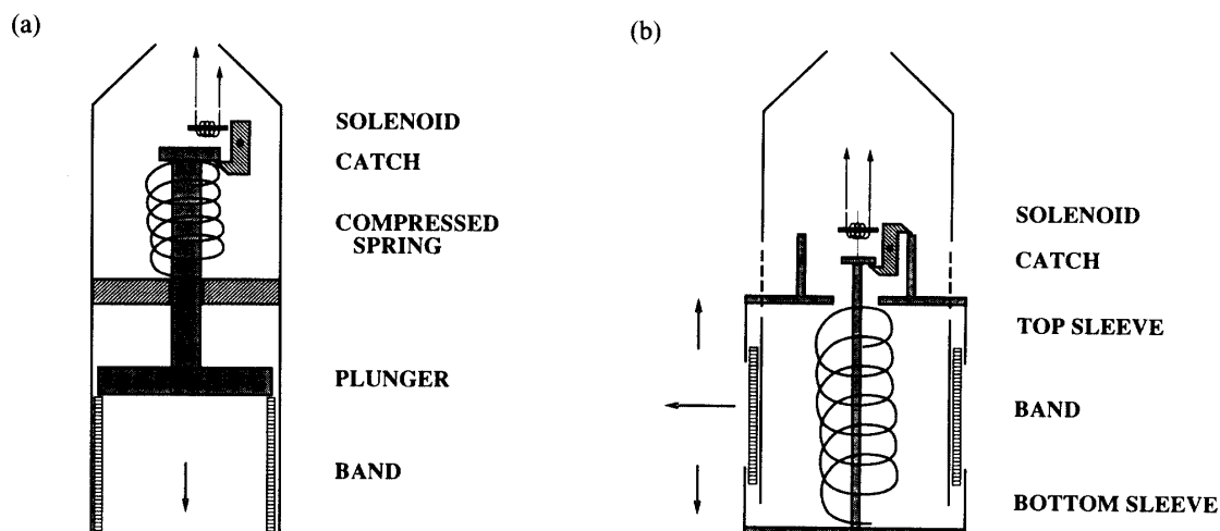
Fig. 1. Schematic of the band injector (a) and suggested alternative (b).
