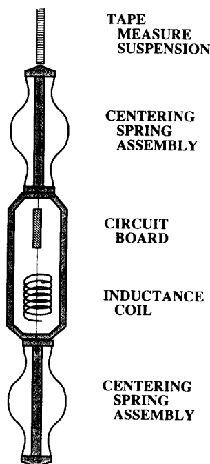
Fig. 2. Schematic of the sensor assembly.
