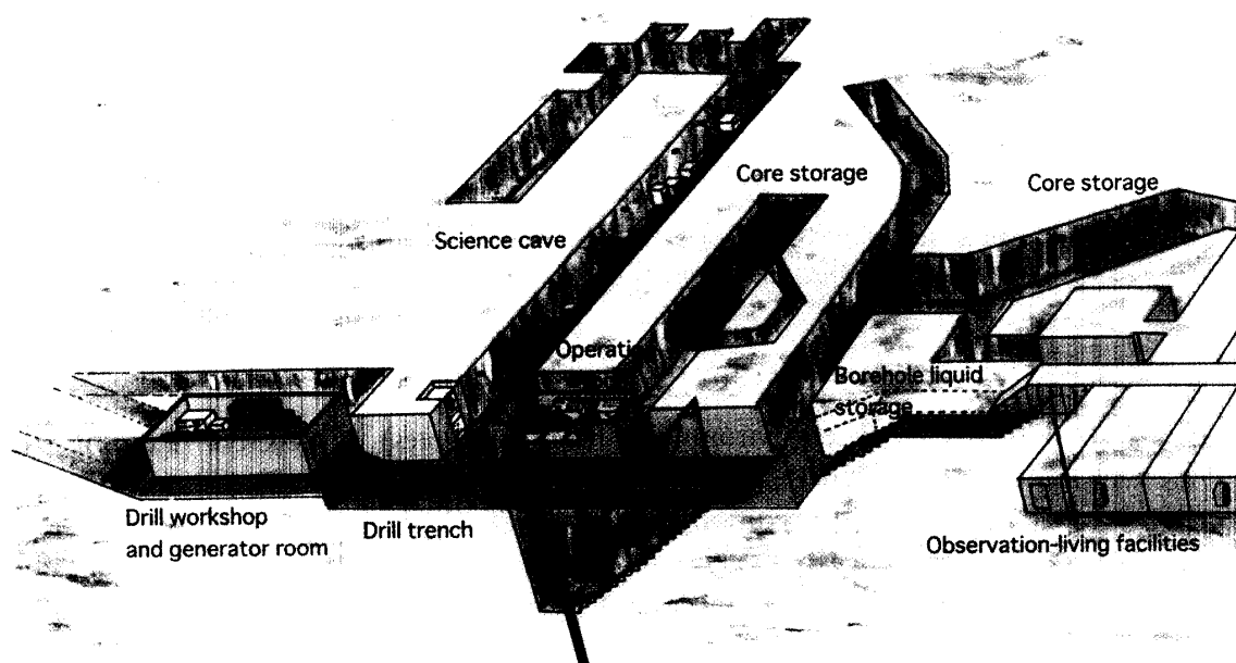
Fig. 1. A Bird's-eye-view of the drilling and related facilities at Dome Fuji Station.
