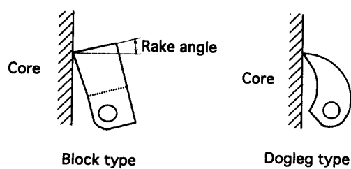
Fig. 5. Schematic of two types of core catcher.
