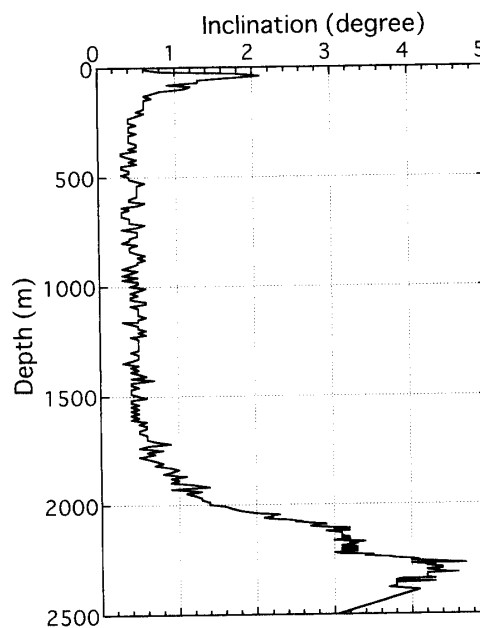
Fig. 13. Profile of borehole inclination.
