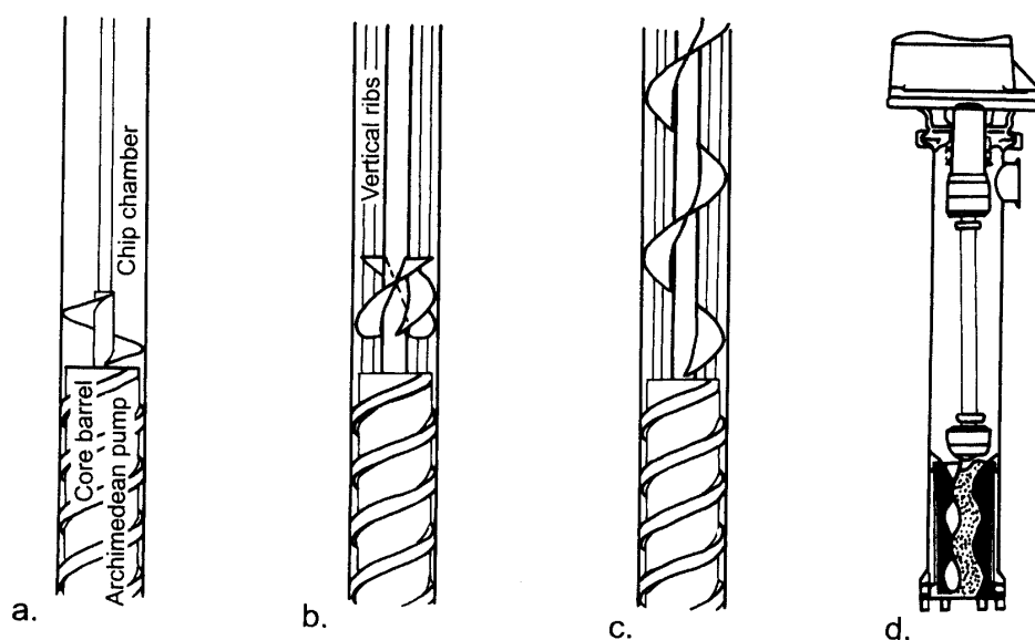
Fig. 1. Four types of pump used for test. a: a one-turn screw booster, b: a three-vane screw pump, c: a conveyer pump and d: a Mohno pump.
