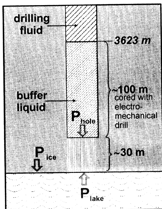
Fig. 2. Schematic of conditions in the near-bottom part of deep Hole 5G-1 before the penetration into Lake Vostok.
