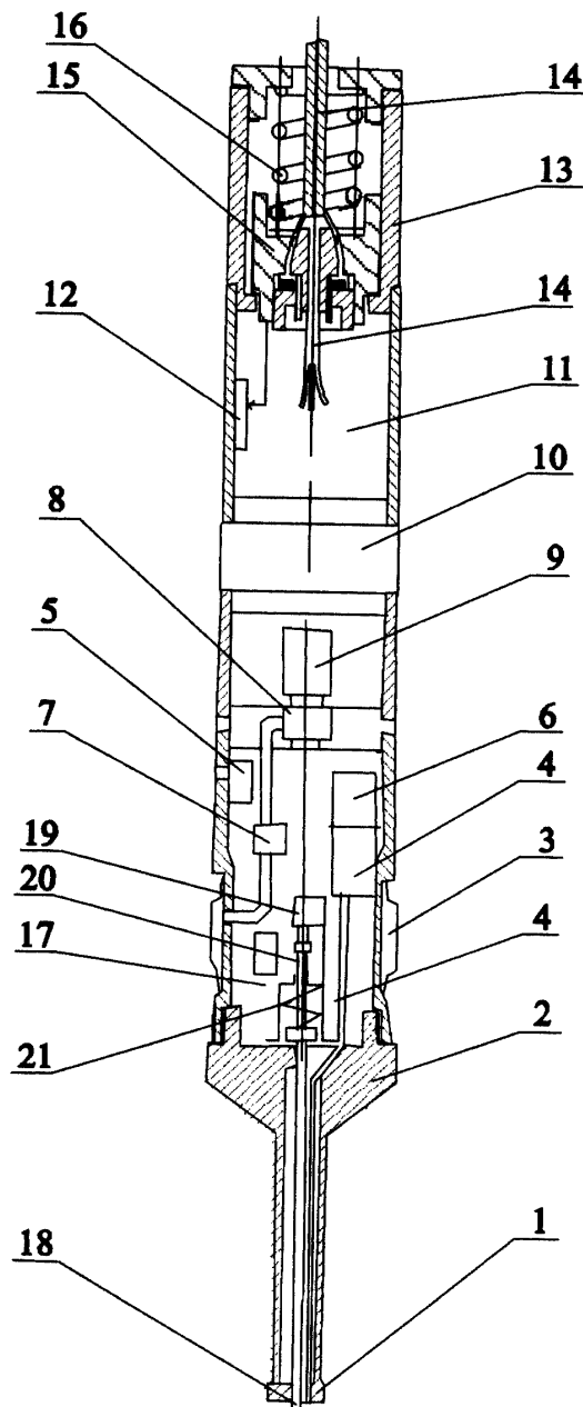
Fig. 3. Schematic of the thermal drill TBPO-132: 1-pilot drill bit, 2-ring drill bit, 3-packer, 4, 5, 6-pressure sensors, 7-valve, 8-pump, 9-driving motor, 10-unit of electronics, 11-electrical compartment, 12-sensor of the load on a hole bottom, 13-cable lock, 14-cable, 15-moveable bush, 16-spring, 17-contact sensor, 18-stock, 19, 20-sensing elements, 21-spring.
