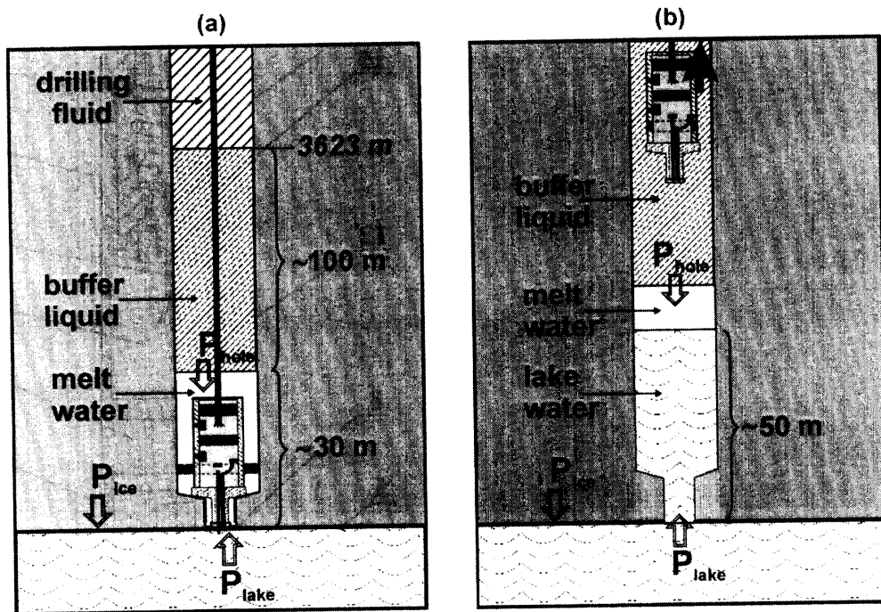
Fig. 4. Schematic of the project realization at the moment the drill tip touches the ice-water interface (a) and during the drill lifting (b).
