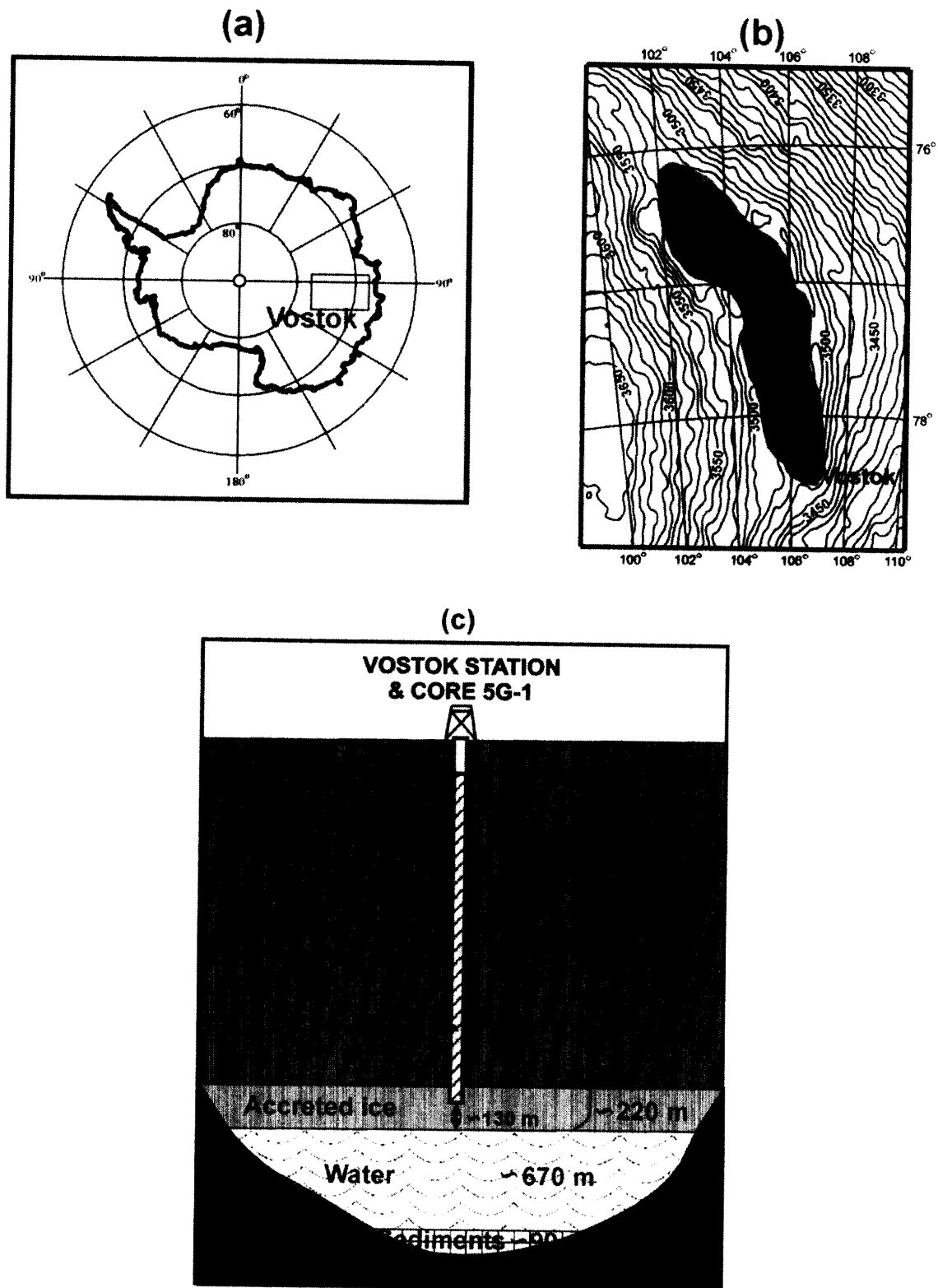
Fig. 1. (a, b) Location of Vostok Station and Lake Vostok. (c) Summary on the deep Hole 5G-1 and Lake Vostok in the vicinity of Vostok Station.
