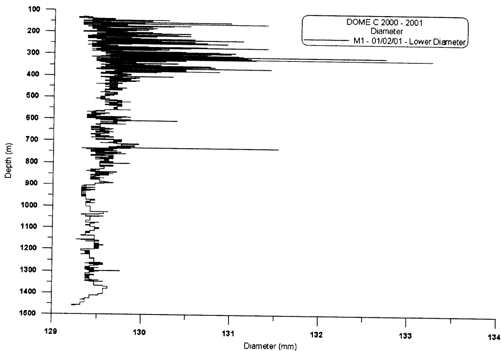
Fig. 9. The average diameter measured at lower pantograph of a borehole logger, in the Dome C second hole in 2001. The record of the measurements starts below the casing. We noticed many accidents at the beginning of the hole due to the mechanical problems. The second part shows a correct drilling operation.
