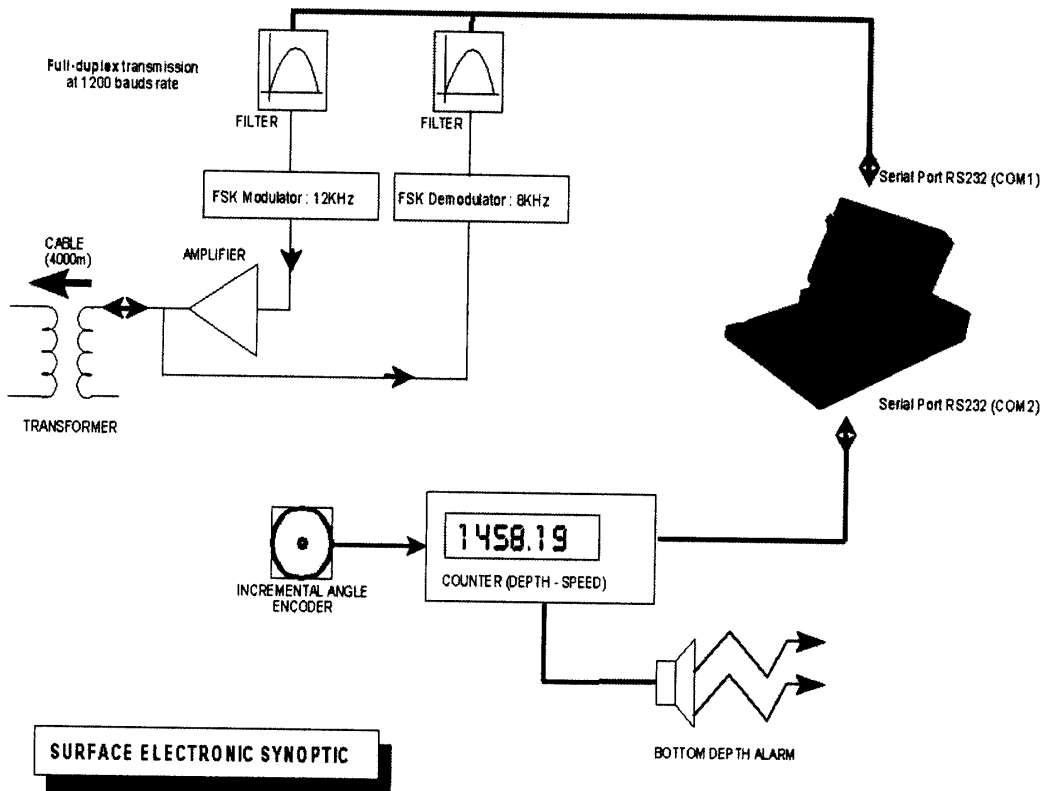
Fig. 5. Surface electronic diagram.
