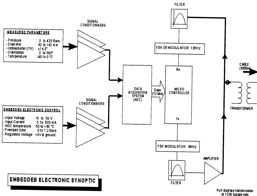
Fig. 2. Embedded electronic diagram.
