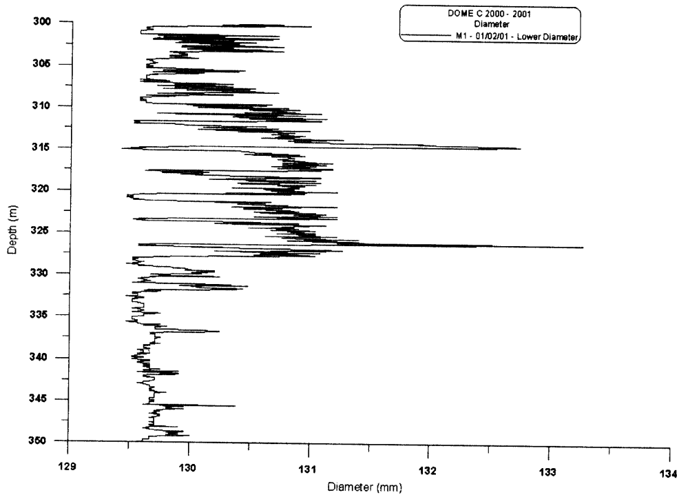
Fig. 8. The average diameter measured at lower pantograph, in the Dome C second hole in 2001. Diameter detail is between 300 and 350 m, when the drilling was disturbed by mechanical problems.
