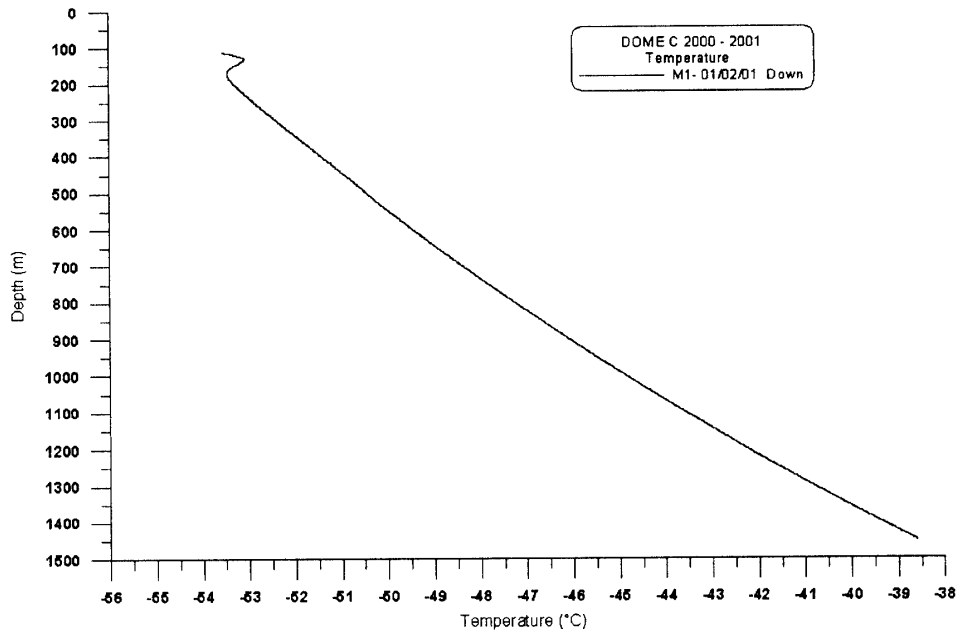
Fig. 10. Temperatures measured in the Dome C second hole in 2001.
