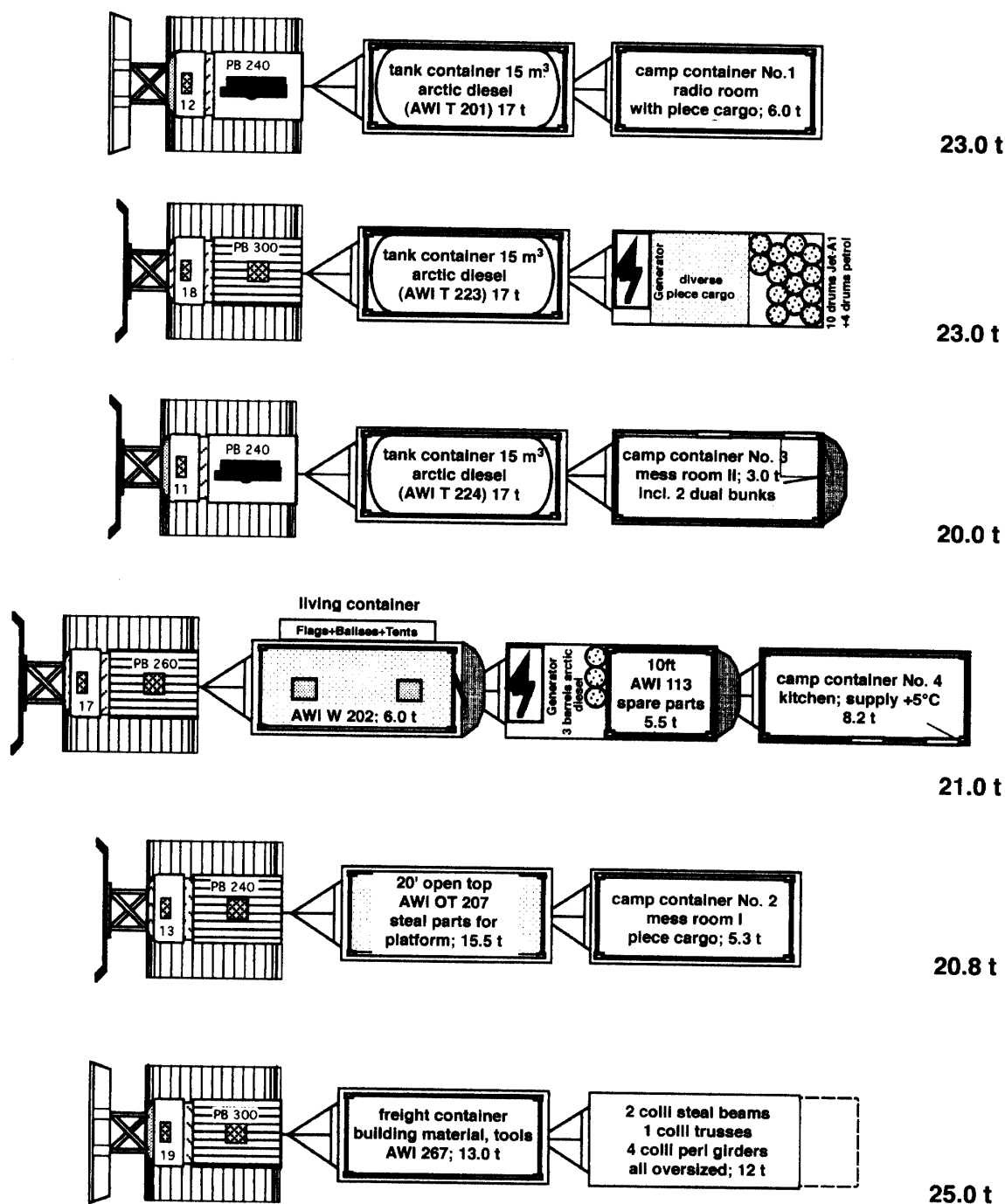
Fig. 2. Load plan for the first traverse of the 1999/2000 season ex Neumayer base to Kohnen base. The given weights illustrate the typical payload of about 20 t per sledge train.
