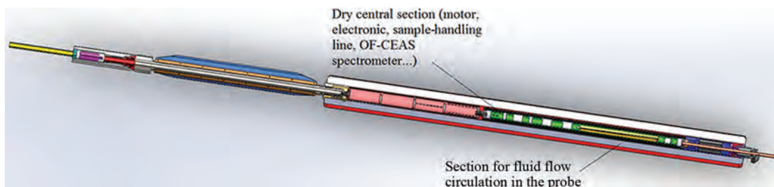
Fig. 2. Internal fluid circulation in the probe.
